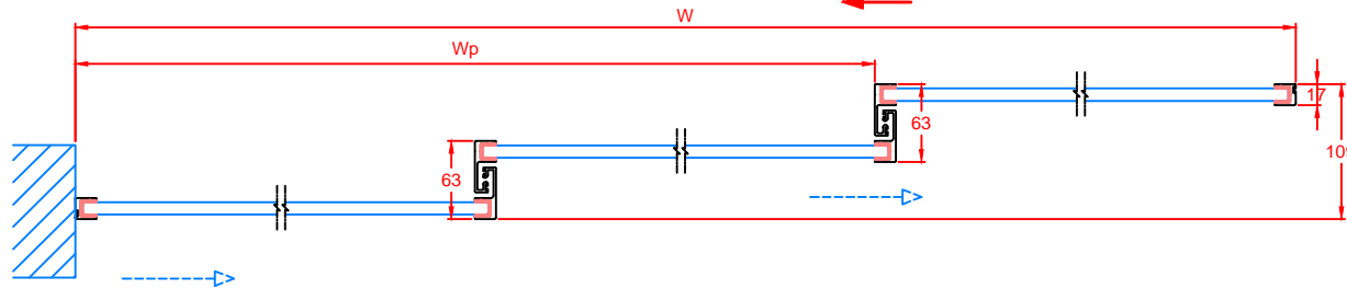
Section B-B
