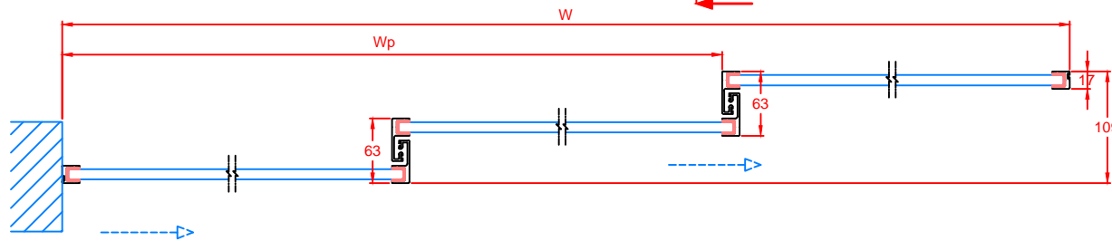
Section B-B
