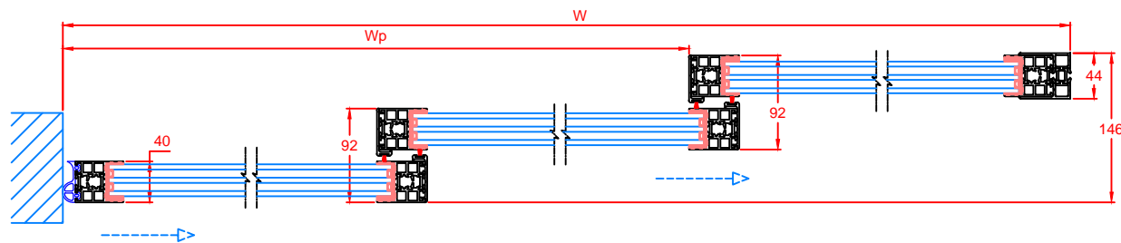
Section B-B
