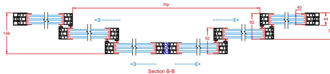
Section B-B
